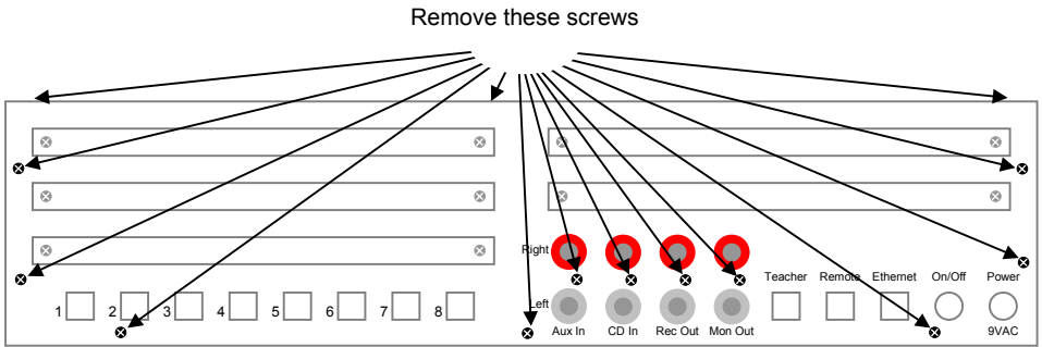
Music Teaching Lab Hub Rear Panel
