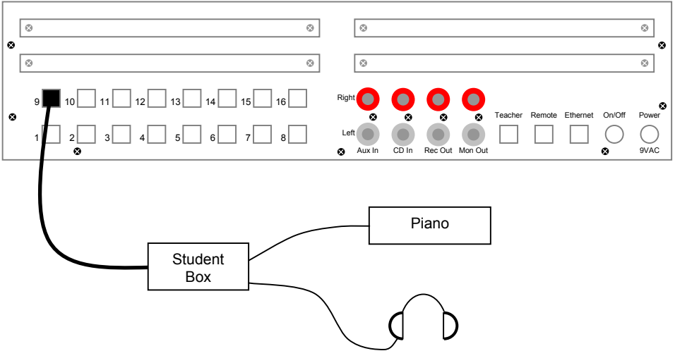
Connecting Student Box to Piano, Hub and Headsets
