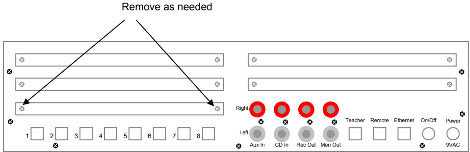
Removing Blank Plate
